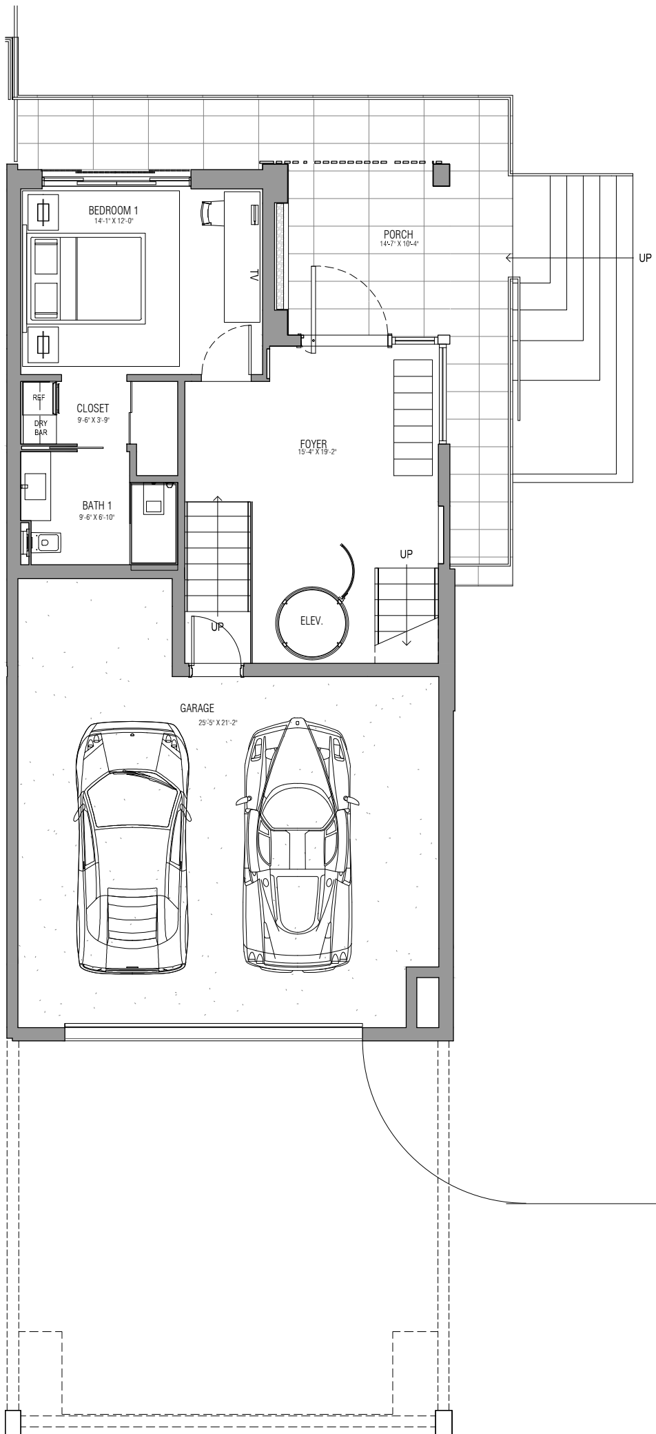
TOWNHOUSE TYPE B GROUND FLOOR PLAN SCALE \frac{1}{8}" = 1'-0"
